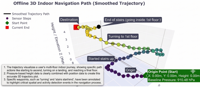
Fig. 2. Reconstructed 3D indoor multi-floor walking trajectory generated on the i.MX RT1064[cite: 9]. The trajectory highlights critical spatial waypoints, including the origin ( Z = 0.00\text{ m} , P_0 = 910.48\text{ hPa} ), stair ascension, landing turn, and arrival at the 1st floor destination[cite: 9].
